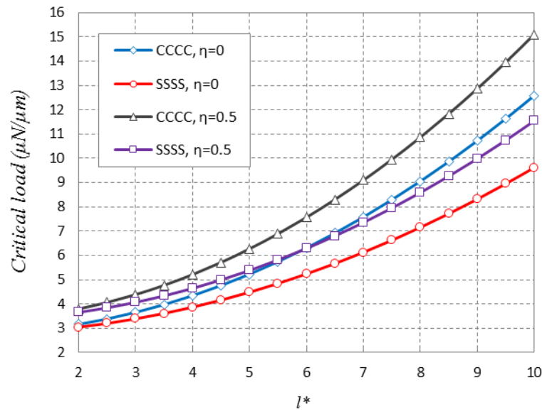
Fig. 6. Variation of the length scale parameter versus the loading type on the critical load in various boundary conditions ( \beta=1 , Lx=20h , kl=k2=1 , T=0.1 , l^*=l/h , m=n=1 , Epoxy)
