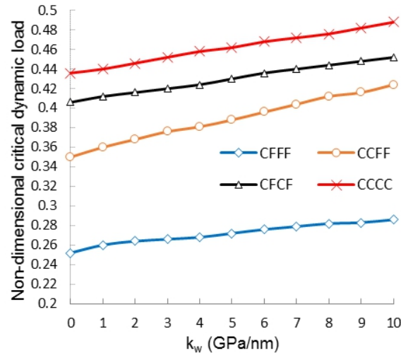
Fig. 7. Winkler stiffness in viscoelastic foundation versus various boundary conditions ( \Omega=2 , C_D=0.1 , e_0a=2nm , kl=1 ; k_2=0 , \beta=1 , k_G=1.13 Pa.m )
