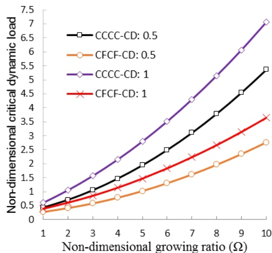
Fig. 6. Growing ratio versus different types of boundary conditions ( eoa=2\text{nm} , k_1=1 ; k_2=0 , \beta=1 ).
