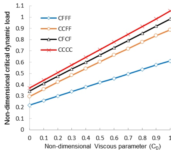
Fig. 8. Viscous damper in viscoelastic foundation versus various boundary conditions ( \Omega=2 , e_0a=2nm , kl=1 ; k_2=0 , \beta=1 , k_G=1.13 Pa.m , k_w=1.13GPa/nm ).
