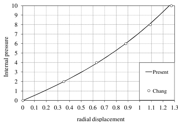
Fig. 6. Radial deflection of cylindrical shell under internal pressure
