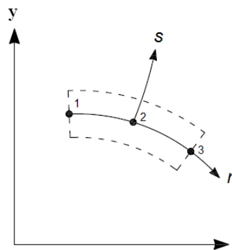
Fig. 1. Isoparametric 1D three-noded element
