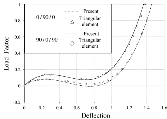
Fig. 10. Deflection of conical shell under ring load
