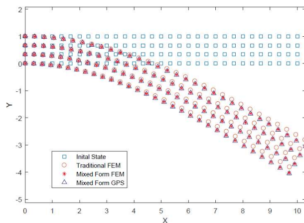
Fig. 4. Deformation comparison among different methods (scaled by 1000)
