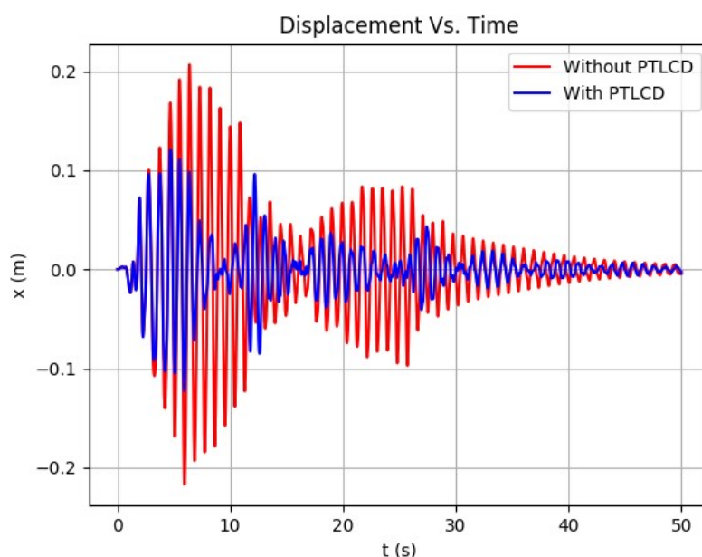
Fig. 4. Dynamic response of a 10-story building under El Centro earthquake with and without PTLCD.
