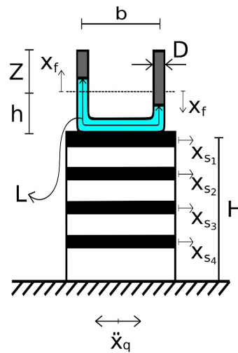
Fig. 1. Geometric parameters of the structure-PTLCD system.
