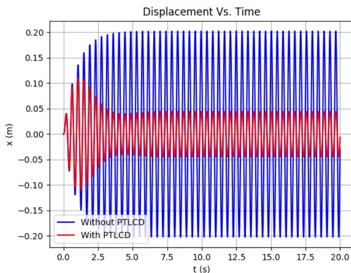
Fig. 3. Dynamic response of a 5-story building under harmonic excitation with and without PTLCD.
