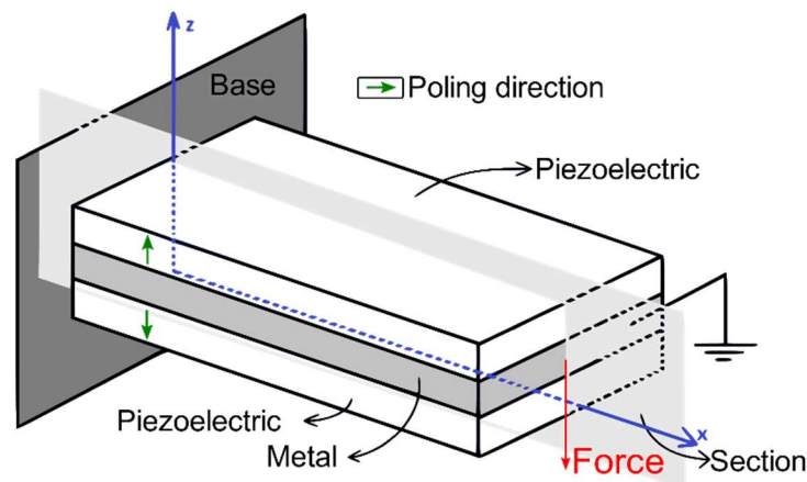
Fig. 1. Piezoelectric harvester model
