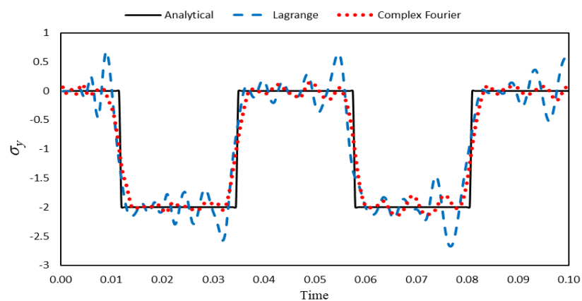
Fig. 10. Normal stress time history at point A.
