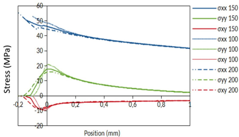
Fig. 19. Stresses at the interface, 2D modeling W_{adh} = 4 mJ (corresponding to 125 N for 1.6 thickness substrate), for 3 dimensions of the fillet.
