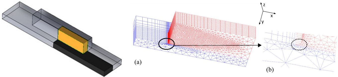
Fig. 3. Modeling of a quarter of the specimen. The adhesive is bounded on the top of the 2024 plate.
