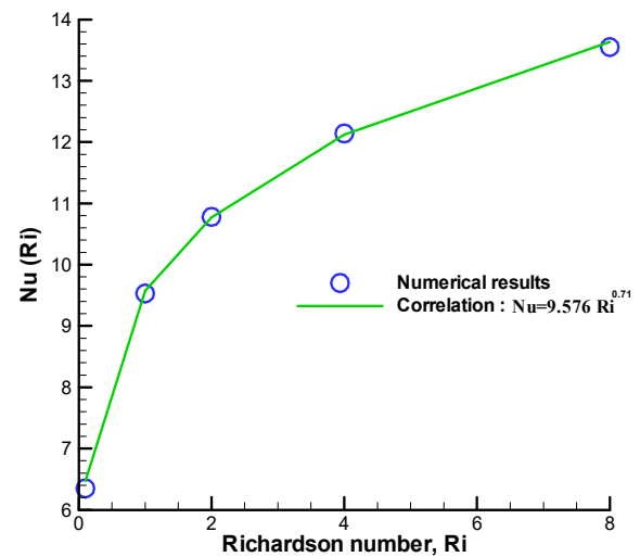
Fig. 16. Variation of Nu(Ri) with Ri in the established zone: comparison between numerical results and correlation.
