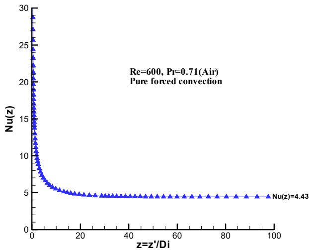
Fig. 13. Variation of Nu(z) with z'/Di at Ri=0 and Re = 600 (for air).
