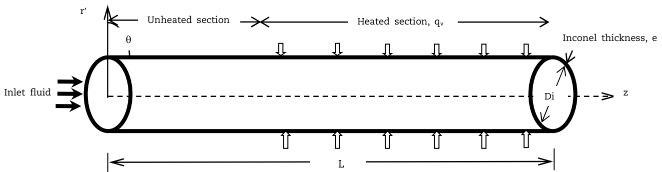
Fig. 1. Horizontal duct with boundary conditions.
