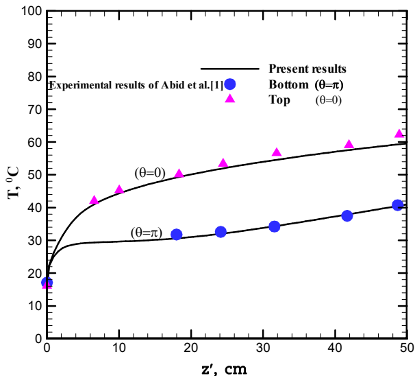
Fig. 3. Comparison of our numerical results and the Abid et al. experimental data [1].
