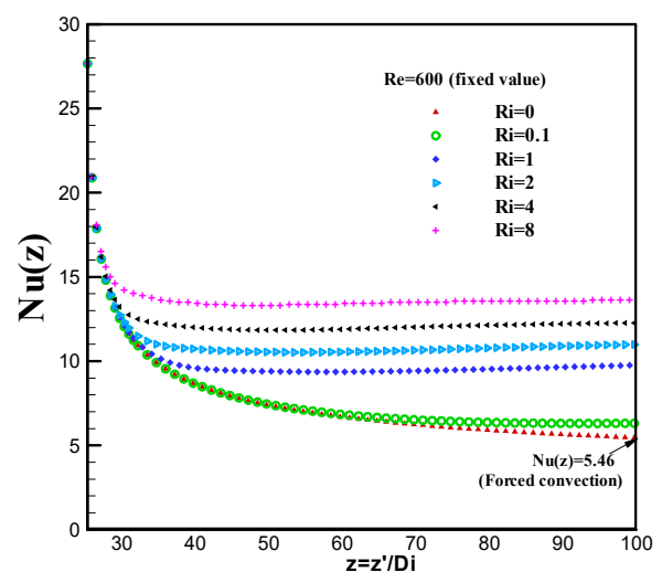
Fig. 12. Variation of Nu(z) with z'/Di for various values of Ri , at Re=600 (for water).
