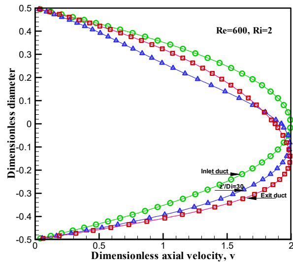
Fig. 9. Axial velocity profiles v with the diameter of the conduit, for different values of z'/D_i at Ri=Gr/Re^2=2 and Re=600 .
