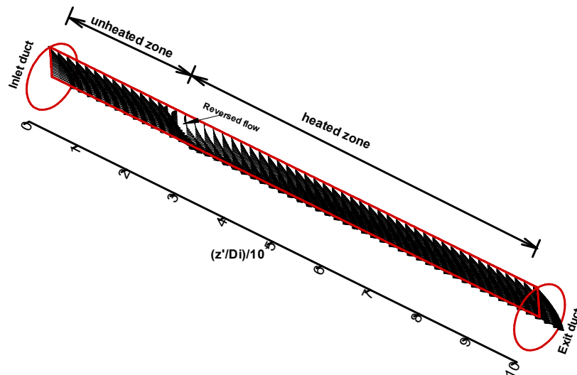
Fig. 5. Velocity vector field in the r - z plane along the horizontal duct, showing the reversed flow, for Re=10 , Gr=10^5 .
