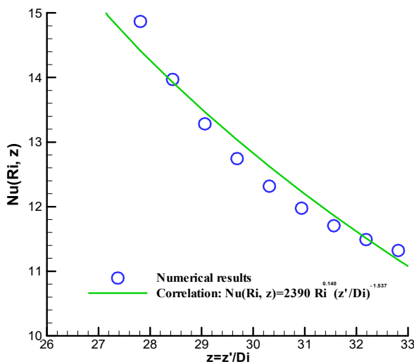
Fig. 15. Variation of the peripherally averaged local axial Nusselt number Nu(Ri, z) as a function of z'/Di in the entry zone: comparison between numerical results and correlation.
