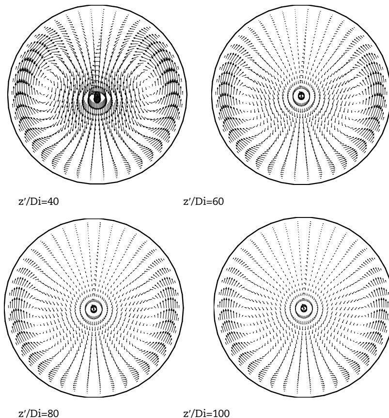
Fig. 8. Velocity vectors ( u-w ) in the plane r-\theta for different values of z'/Di (cross-section), at Ri=2 and Re=600 .
