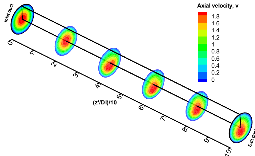
Fig. 7. Contours of the axial velocity v for different values of z'/Di , at Ri=2 and Re=600 .
