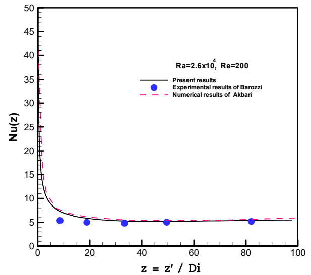
Fig. 4. Comparison of our results with those of Akbari et al. [28] and Barozzi et al. [27] experimental data.
