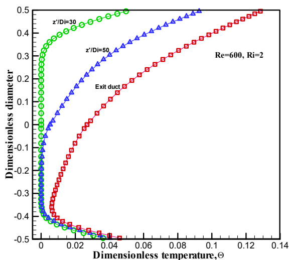
Fig. 11. Profiles of the temperature \Theta with the tube diameter, for various values of z'/Di at Ri=2 and Re=600 .
