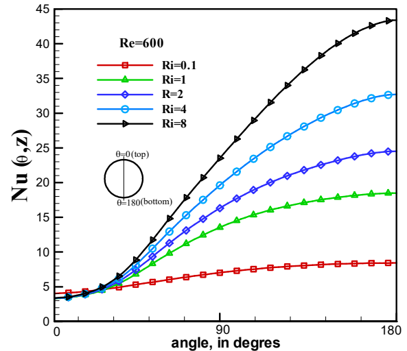
Fig. 14. Variation of Nu(\theta, z) , at z'/Di = 80 (in the established zone), as a function of angular coordinate \theta for different values of Ri , at Re=600 .
