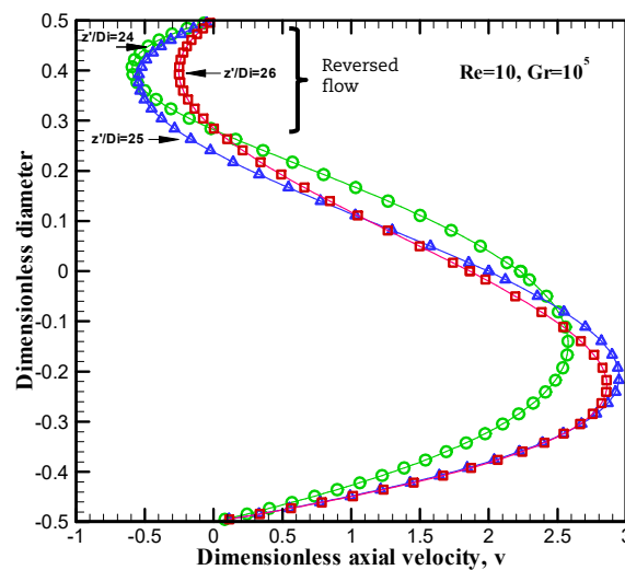
Fig. 6. The axial velocity profiles v with the diameter of the tube, for various values of z'/Di , showing the reversed flow (represented by negative values of the axial velocity near the top wall), at Re=10 and Gr=10^5 .
