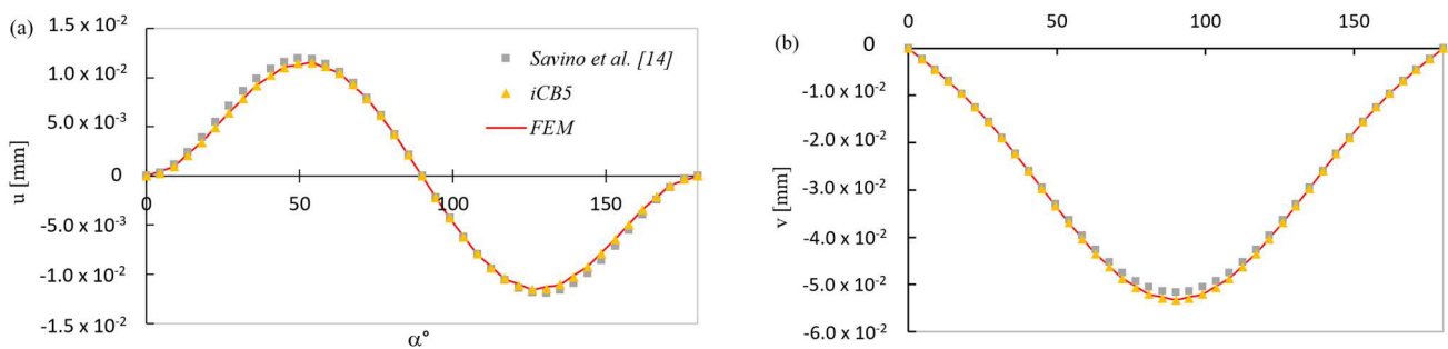
Fig. 7. Comparison along the arch axis of iFEM solution (Savino et al. [14], iCB5) to FEM analysis for the displacements u (a) and v (b), and strains \epsilon (c) and \chi (d).
