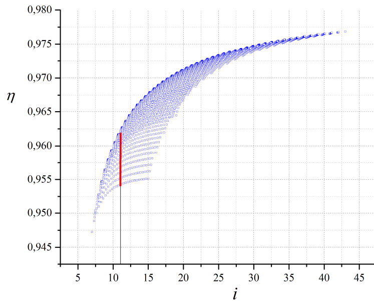
Fig. 7. Scatter chart showing the possible values of the efficiency ratio as a function of the overall transmission ratio i for the S16WN(E) PGT in the interval t_I = 1,5 \dots 6 and t_{II} = 1,5 \dots 6 .
