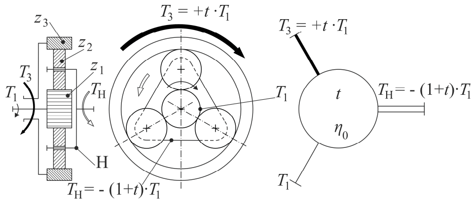
Fig. 4. Cross-section (left) and frontal view (center) of simple component gear train with Wolf-Arnaudov symbol and specific torques acting on the shafts (right) [18].
