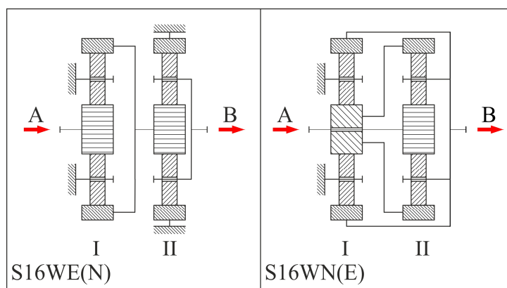
Fig. 13. Kinematic schemes of the S16WN(E) and S16WE(N) planetary gear trains.
