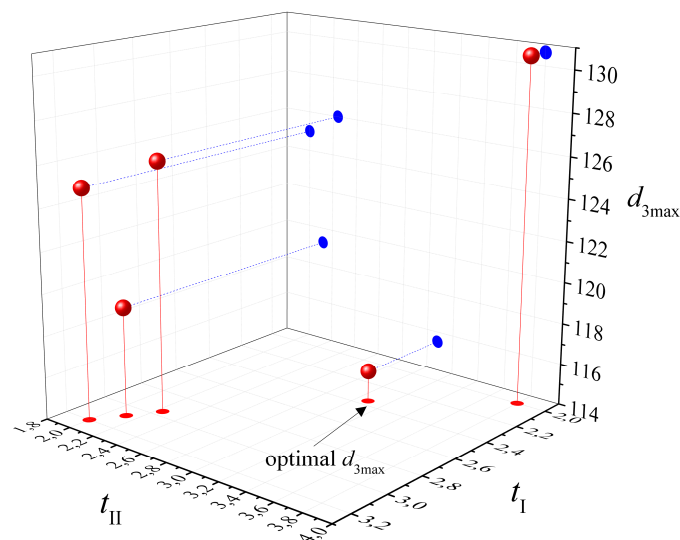
Fig. 10. Influence of numerically determined ideal torque ratios on the maximum ring gear reference diameter of the S16WN(E) gear train.
