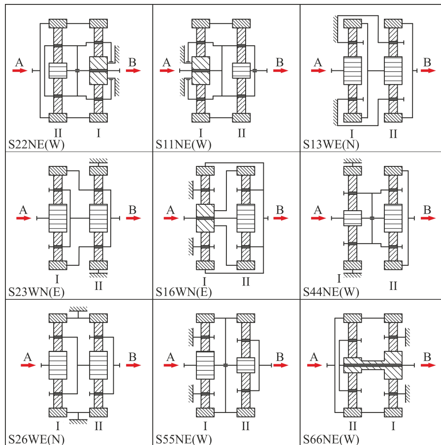
Fig. 11. Kinematic schemes of valid PGT variants with positive transmission ratios.
