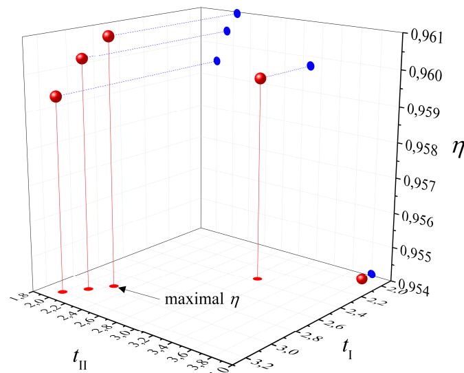
Fig. 9. Influence of numerically determined ideal torque ratios on the efficiency ratio of the S16WN(E) gear train.
