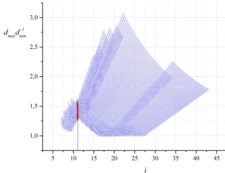
Fig. 8. Diagram of the ratio of the larger and smaller ring gear reference diameter as a function of the transmission ratio for the S16WN(E) PGT in the interval t_I = 1,5 \dots 5 and t_{II} = 1,5 \dots 5 .
