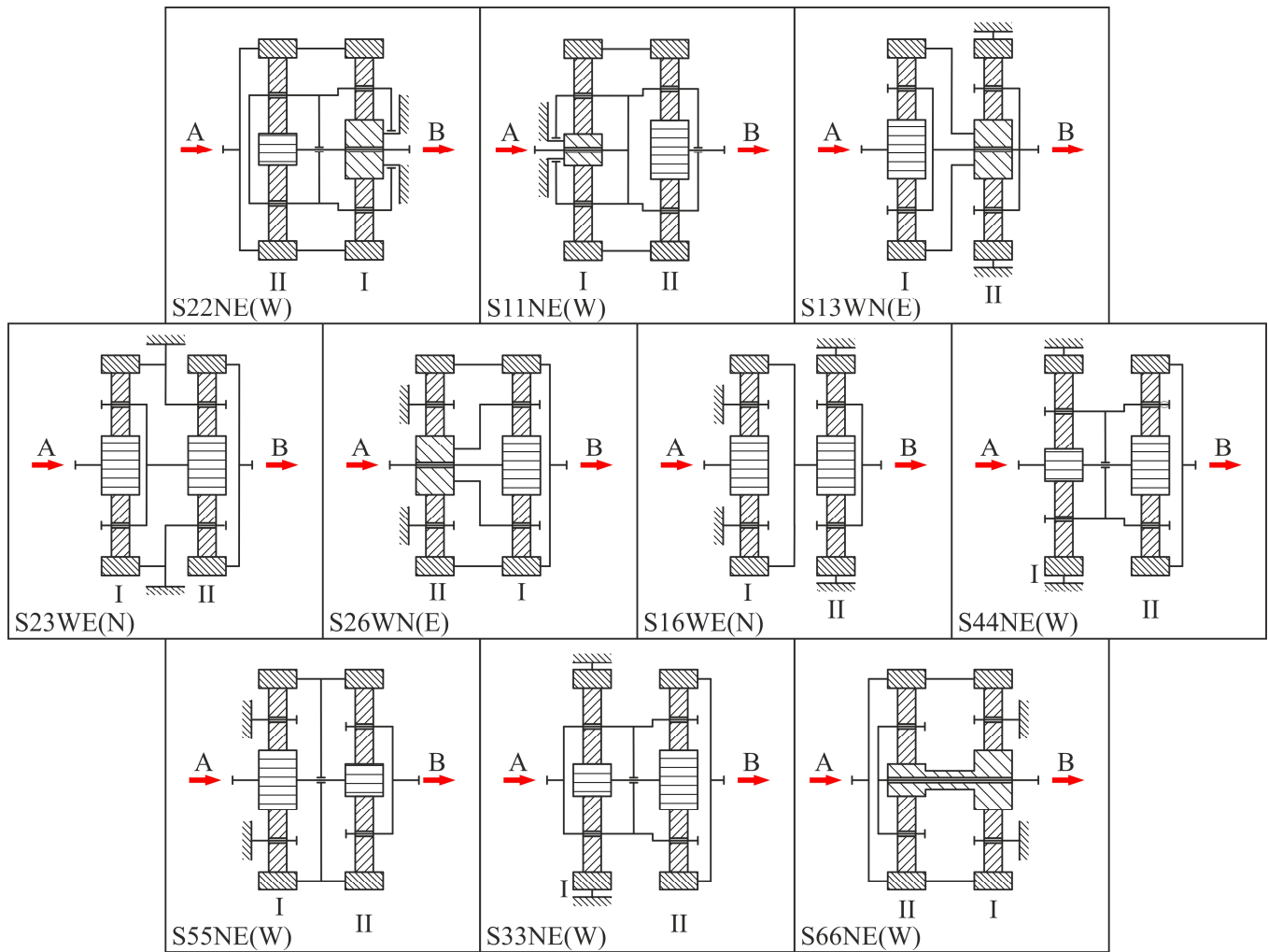
Fig. 12. Kinematic schemes of valid PGT variants with negative transmission ratios.
