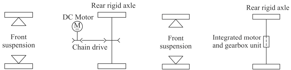
Fig. 2. Mechanical layout of a chain-driven (left) and of a compact drive (right) light electric vehicle.
