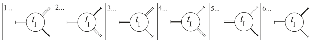
Fig. 5. Symbolic presentation of component planetary gear train connectivity options.
