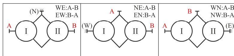
Fig. 6. Schematic overview of layout variant nomenclature according to cardinal points. The red letters A and B are used to denote the external shafts that are used to transfer power to or from the geartrain. The actual layout variant depends on the direction of the power flow being from A to B or from B to A.
