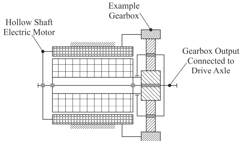
Fig. 3. Schematic layout of a hollow shaft motor and gearbox unit.
