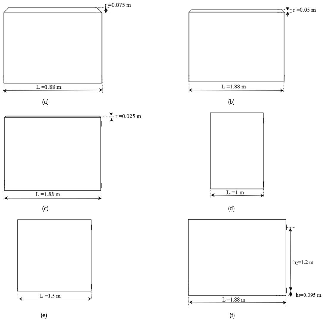
Fig. 2. The computational domain used for the various analyzed scenarios, (a) r = 0.075 \text{ m} and L = 1.88 \text{ m} , (b) r = 0.05 \text{ m} and L = 1.88 \text{ m} , (c) r = 0.025 \text{ m} and L = 1.88 \text{ m} , (d) r = 0 \text{ m} and L = 1 \text{ m} , (e) r = 0 \text{ m} and L = 1.5 \text{ m} , (f) r = 0 \text{ m} and L = 1.88 \text{ m} .
