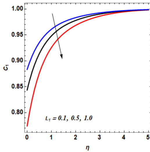
Fig. 10. Influence of L_1 on C_1(\eta) .
