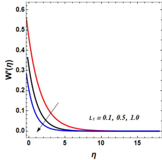
Fig. 9. Impact of L_1 on w'(\eta) .
