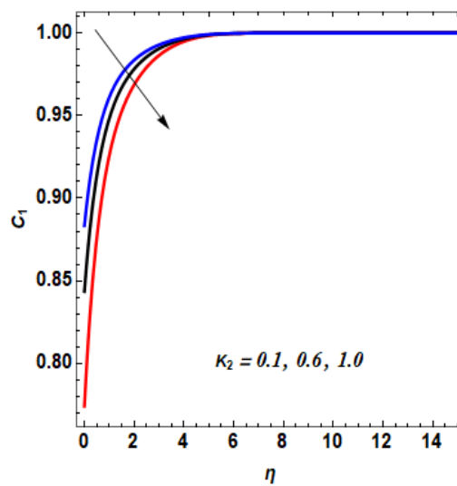
Fig. 20. Influence of k_2 on C_1 .
