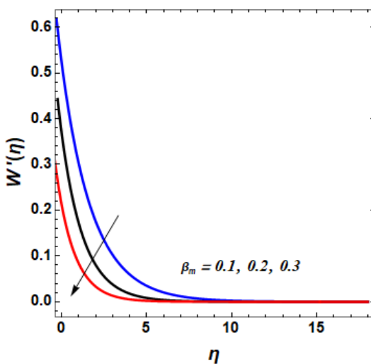
Fig. 6. Impact of \beta_m on w'(\eta) .
