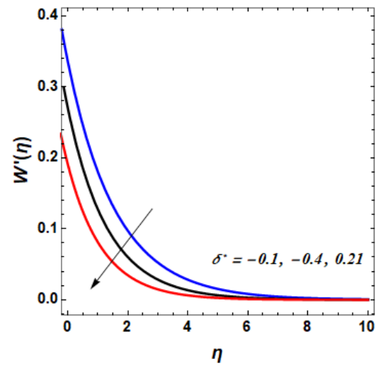
Fig. 11. Impact of \delta^* on w'(\eta) .
