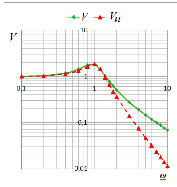
Fig. 6. Comparison of V and V_d coefficients varying depending on frequency for \psi = 4 , \bar{J} = 1 , \bar{k} = 0.1 .
