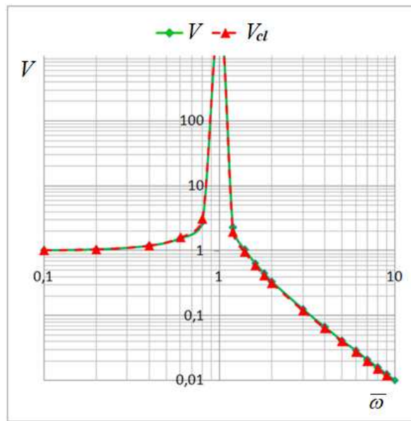
Fig. 3. Comparison of V and V_{cl} coefficients varying depending on frequency with \psi = 0 , \bar{J} = 1 , \bar{k} = 0.1 .
