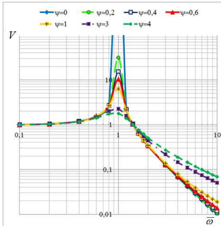
Fig. 2. Diagram of the dependence of the torque growth coefficient on the dimensionless coefficient of the system oscillation frequency for different values of the coupling relative damping coefficient ( \psi ).
