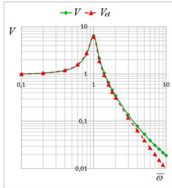
Fig. 5. Comparison of V and V_d coefficients varying depending on frequency for \psi = 1 , \bar{J} = 1 , \bar{k} = 0.1 .
