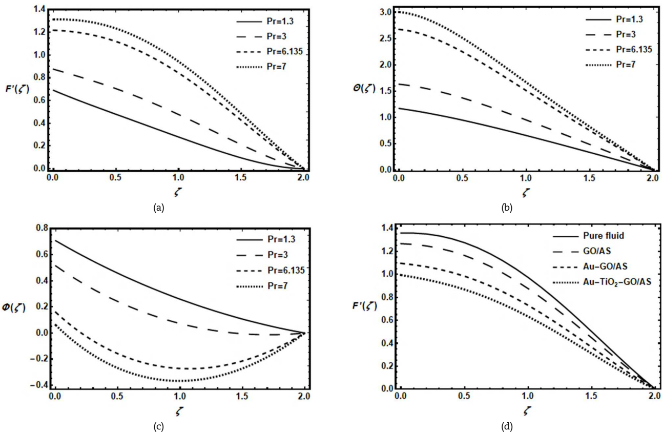
Fig. 7. Variation of Prandtl number and volume ratio of solid nanoparticles via velocity, temperature, and concentration profiles.
