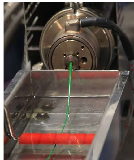
Fig. 1. (a) THSN flow through slandering stretching cylinder, (b) Extrusion cooling process.
