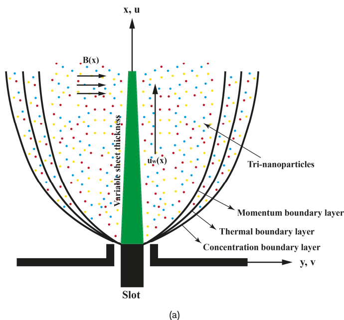
Fig. 1. (a) THSN flow through slandering stretching cylinder, (b) Extrusion cooling process.
