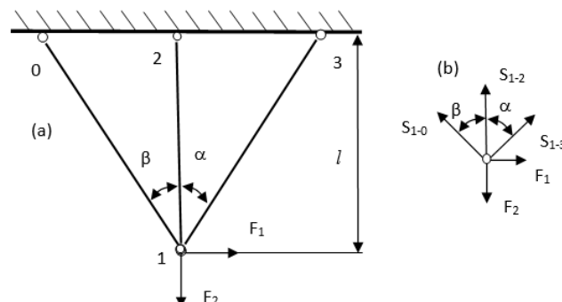
Fig. 1. Two DOF structure: (a) model of structure, (b) node 1.
