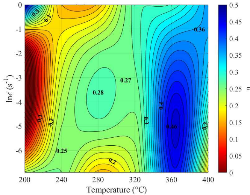
Fig. 3. Power dissipation efficiency map of the extruded Mg-1Zn-0.2Ca alloy at a true strain of 0.7. The strain rate axis is expressed as \ln \dot{\epsilon} , where \dot{\epsilon} is strain rate.
