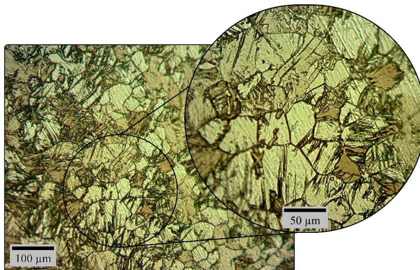
Fig. 1. Optical microstructure of the as-extruded Mg–1Zn–0.2Ca alloy, observed on the plane normal to the extrusion direction. The inset shows a higher-magnification view of the circled area.
