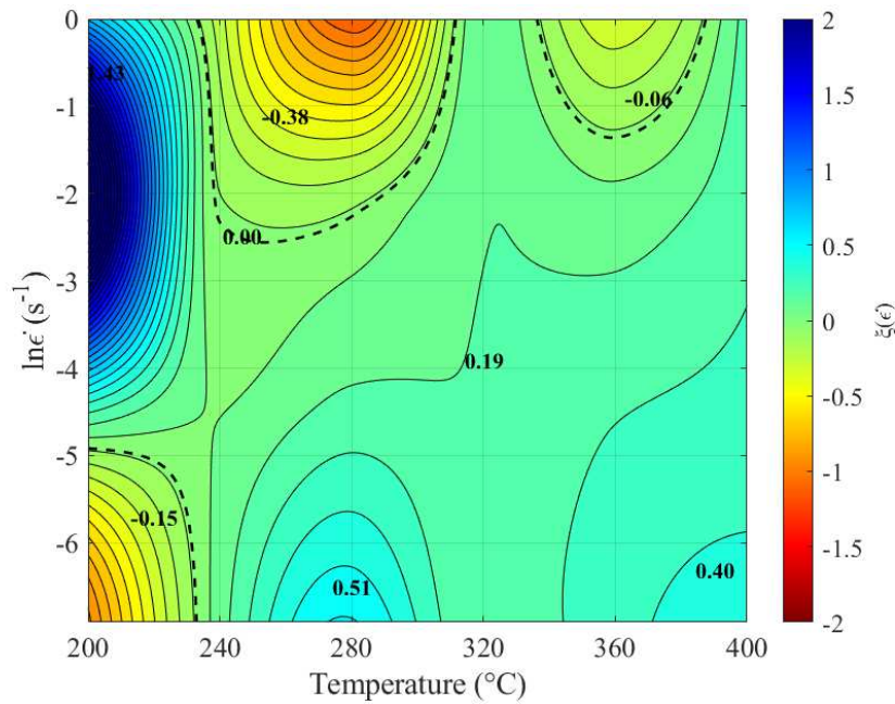
Fig. 4. Flow instability map of the extruded Mg-1Zn-0.2Ca alloy at a true strain of 0.7 based on the \xi criterion. Dashed boundaries define the boundary of the predicted instability domain.
