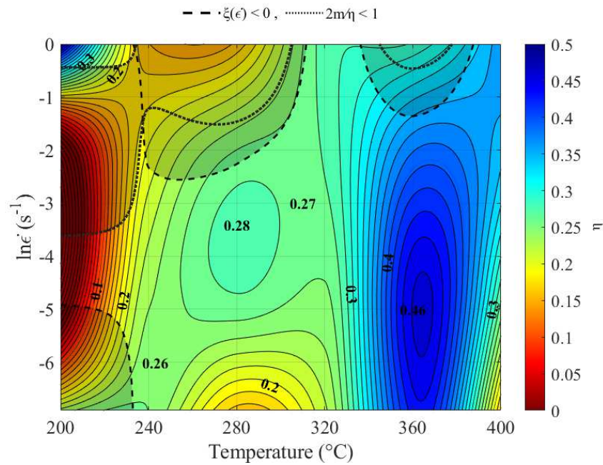
Fig. 6. Processing map of the extruded Mg-1Zn-0.2Ga alloy at a true strain of 0.7. Color contours represent the power dissipation efficiency, \eta , while dashed and dotted boundaries define the boundary of the predicted instability domain by the \xi and 2m/\eta criteria, respectively.
