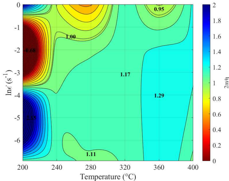
Fig. 5. Flow stability map of the extruded Mg-1Zn-0.2Ca alloy at a true strain of 0.7 based on the 2m/\eta criterion. Dashed boundaries define the boundary of the predicted instability domain.
