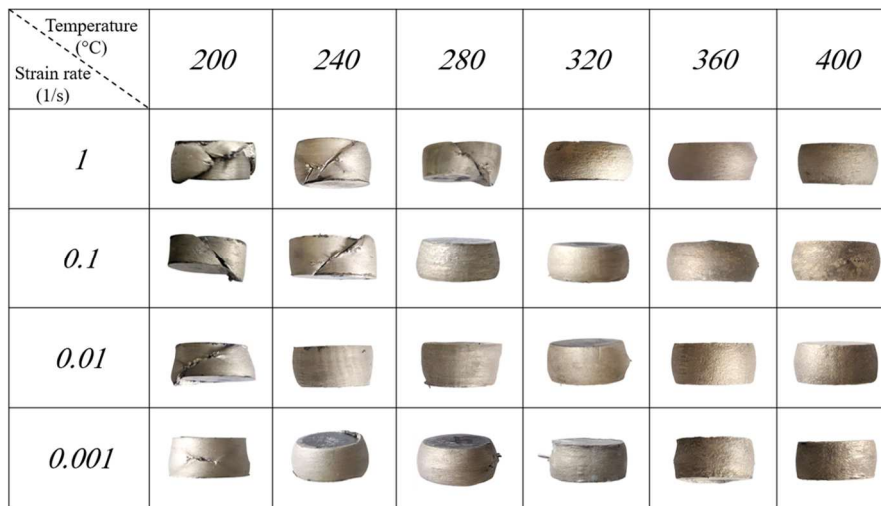
Fig. 7. Macroscopic appearance of the extruded Mg-1Zn-0.2Ca specimens after compression at temperatures of 200–400 °C and strain rates of 0.001–1 s -1 . Cracking is observed at all strain rates at 200 °C, at 0.1–1 s -1 at 240 °C, and at 1 s -1 at 280 °C. No obvious macroscopic cracking is visible in specimens deformed at 320–400 °C.
