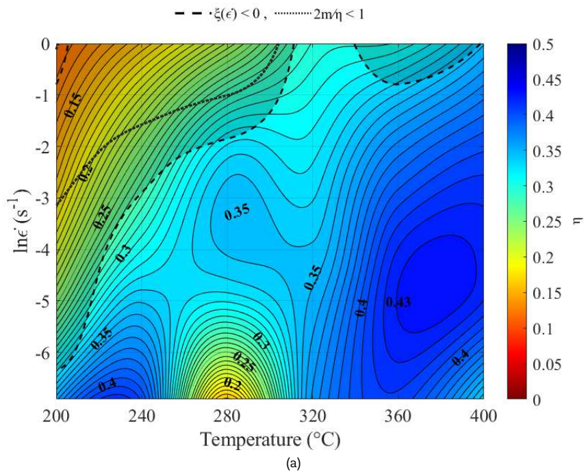
Fig. 9. Processing maps of the extruded Mg-1Zn-0.2Ca alloy at true strains of, (a) 0.3 and (b) 0.5. Color contours represent the power dissipation efficiency, \eta , while dashed and dotted boundaries define the boundary of the predicted instability domain by the \xi and 2m/\eta criteria, respectively.
