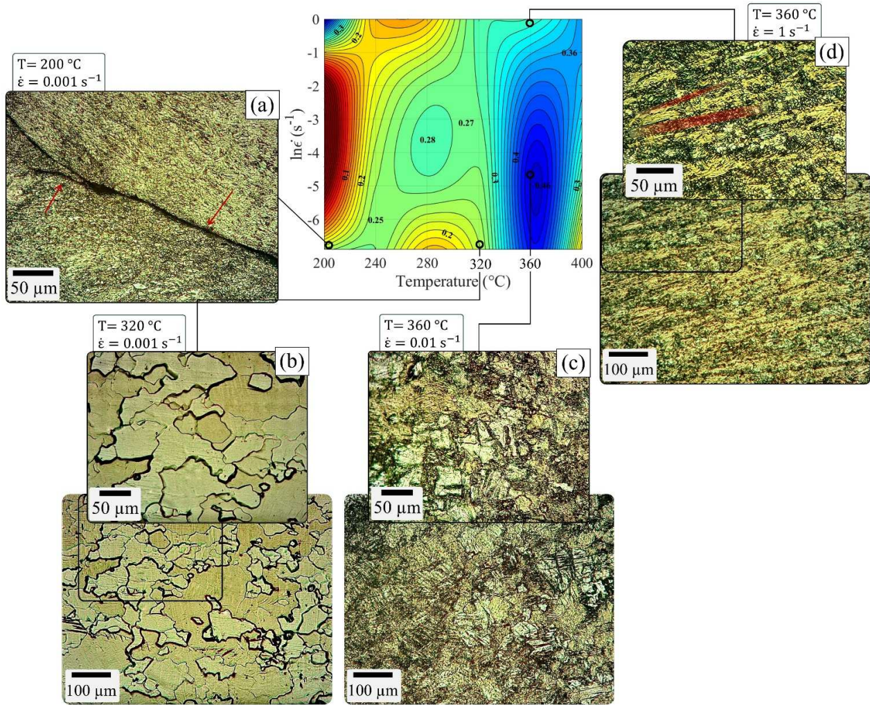
Fig. 8. Optical microstructures at selected conditions marked on the processing map: (a) 200 °C and 0.001 s -1 (crack indicated by arrows), (b) 320 °C and 0.001 s -1 , (c) 360 °C and 0.01 s -1 , and (d) 360 °C and 1 s -1 (localized deformation bands highlighted). The observations were made at the specimen center on sections parallel to the compression axis. In each panel, the smaller image is a higher-magnification view of the area outlined in the larger image.
