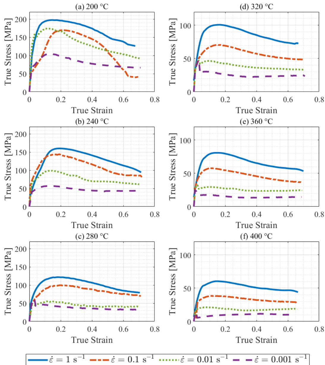
Fig. 2. True stress-true strain curves of the extruded Mg-1Zn-0.2Ca alloy obtained at temperatures of 200–400 °C and strain rates of 0.001, 0.01, 0.1 and 1 s -1 .
